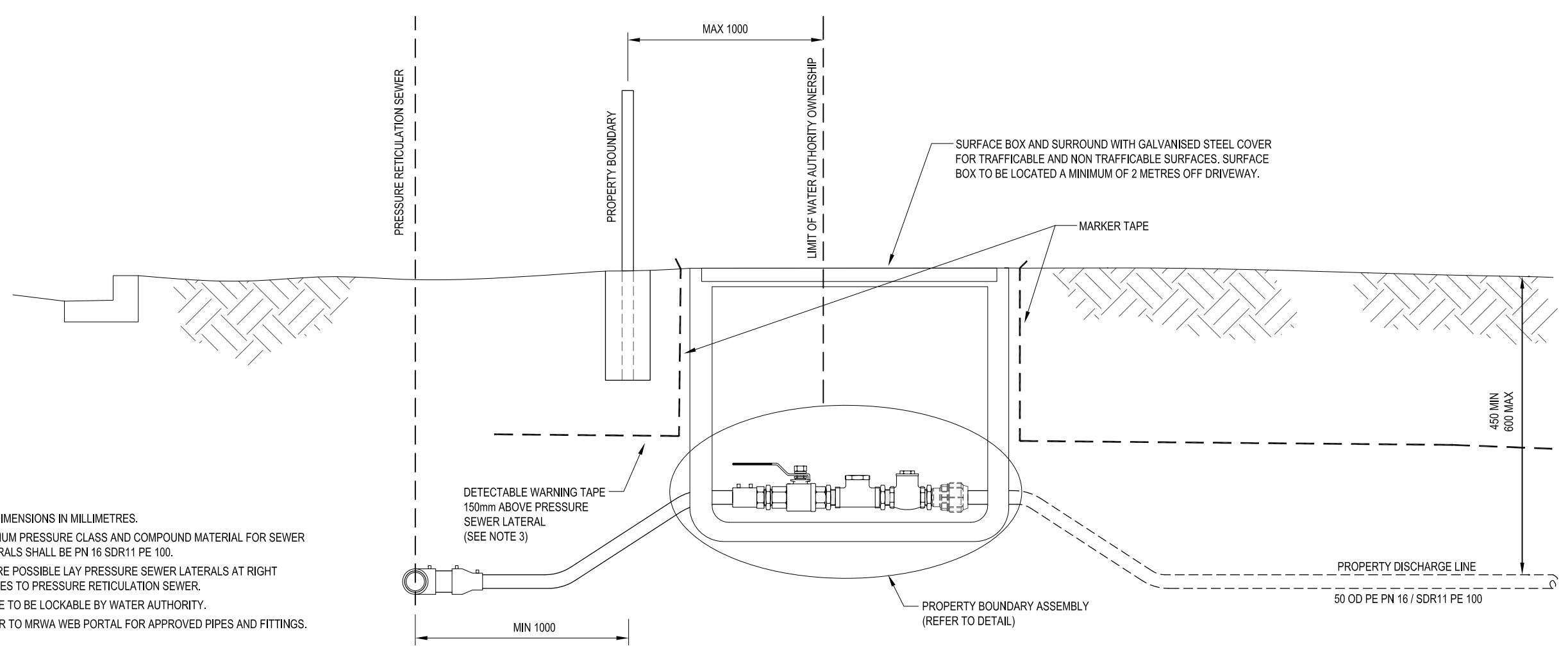
TYPICAL ARRANGEMENT - SECTION NOT TO SCALE
