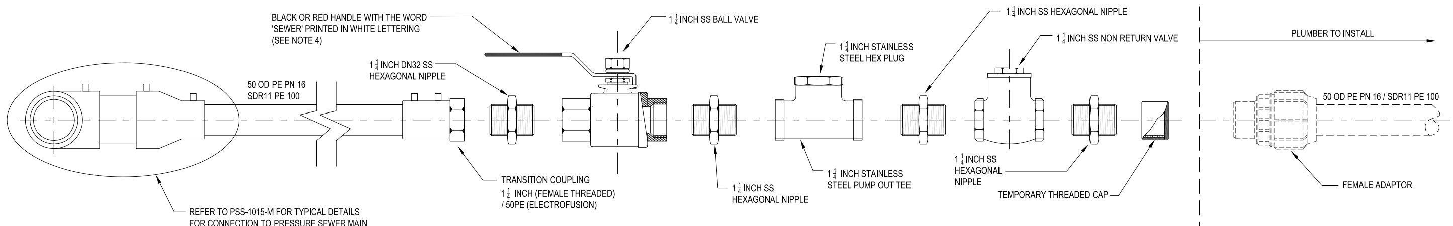
DETAIL - PROPERTY BOUNDARY ASSEMBLY NOT TO SCALE
