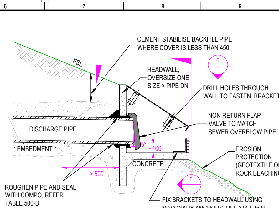
FIGURE 406-B: SEWER OVERFLOW TO WATERWAY (SECTION)
