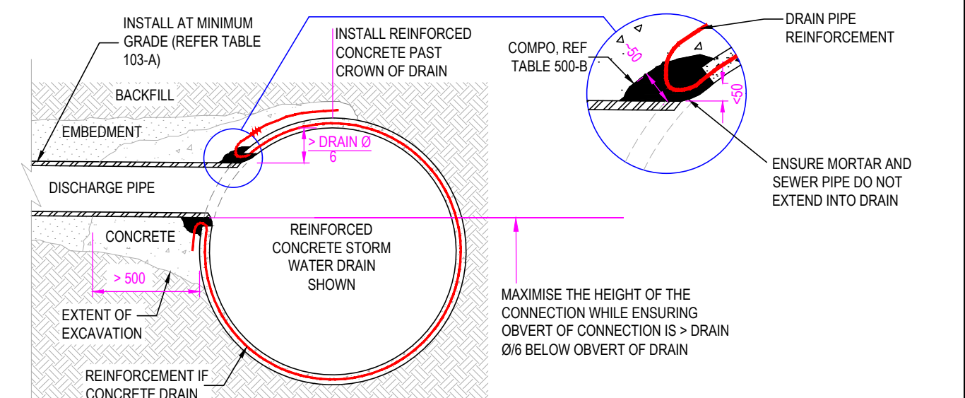
FIGURE 406-F: SEWER OVERFLOW TO STORM WATER DRAIN CONNECTION
