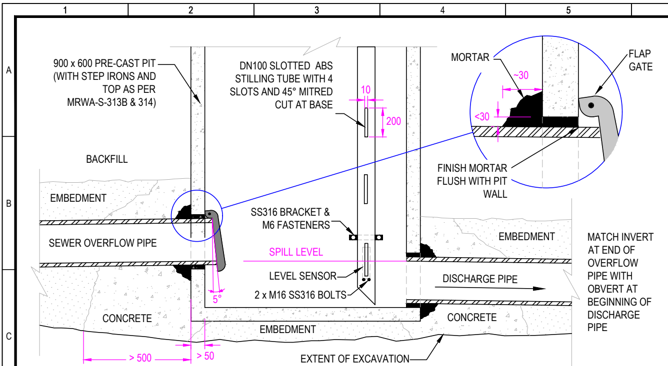
FIGURE 406-A: SEWER OVERFLOW MONITORING PIT (SECTION)
