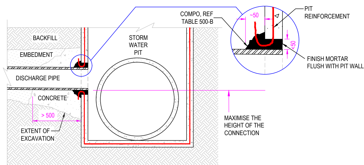
FIGURE 406-E: SEWER OVERFLOW TO STORM WATER PIT CONNECTION
