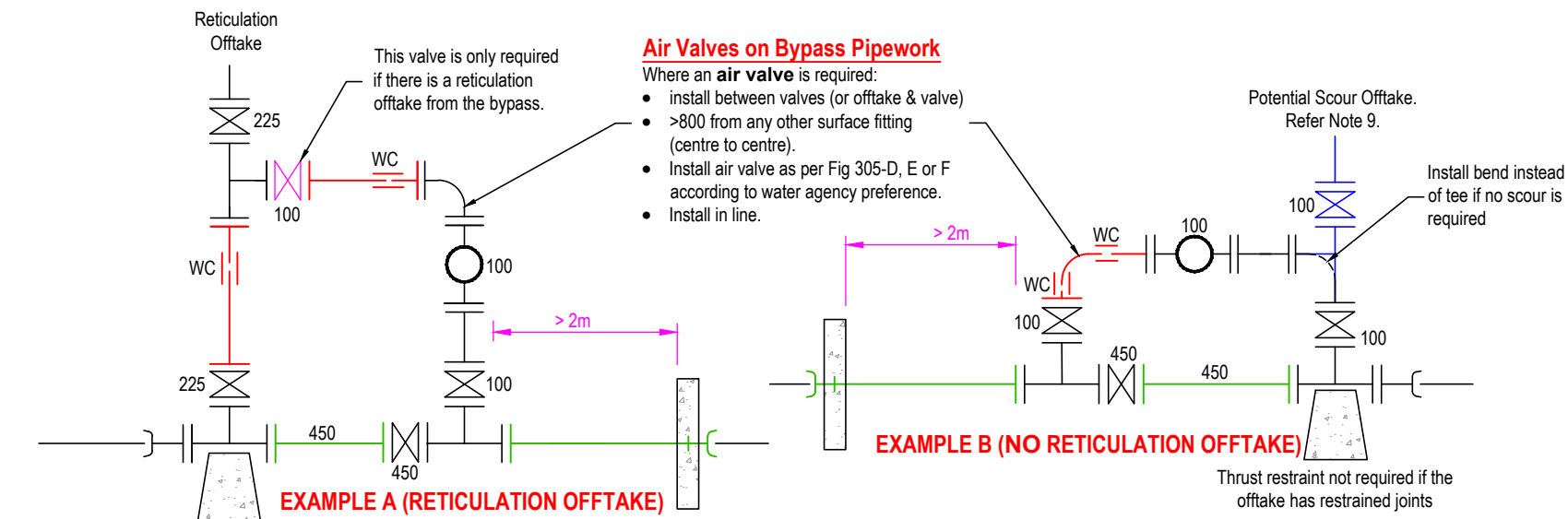
FIGURE 105-B: SOCKET / SPIGOT DISTRIBUTION MAINS (DI or FW-GRP)
