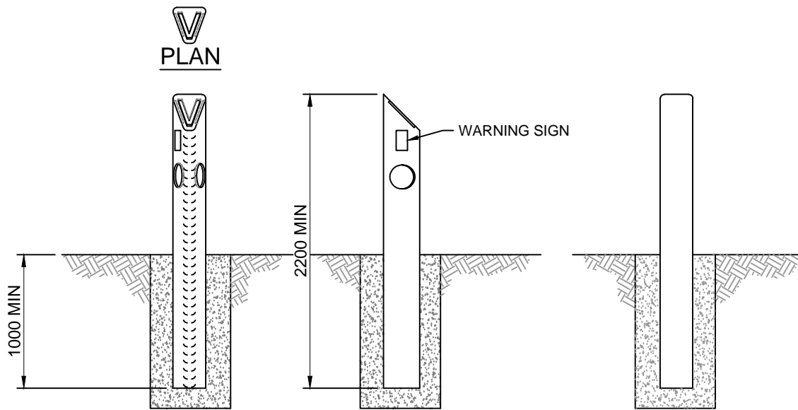
MARKER POST - TYPICAL
