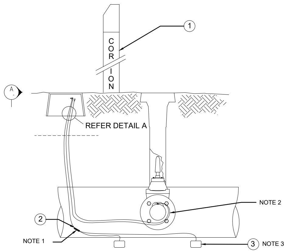
SIDE ELEVATION
