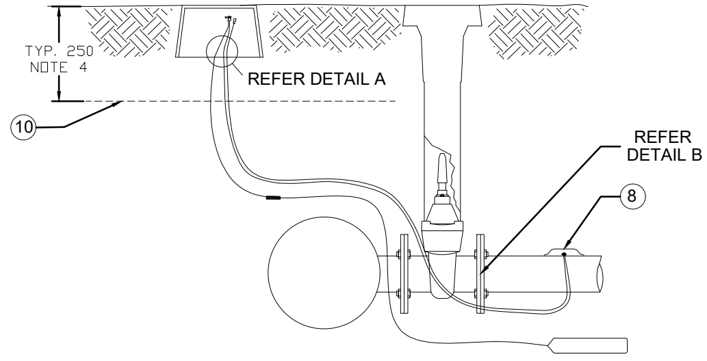
SECTION A
